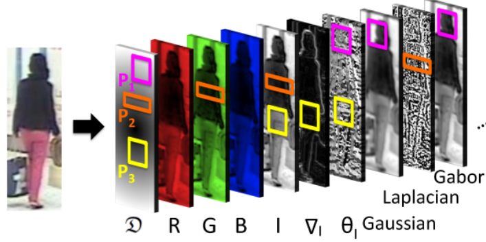
Figure 6.6: A meta covariance feature space. Example of three different covariance features. Every covariance is extracted from distance layer ( \mathfrak{D} ) and three channel functions (e.g. bottom covariance feature is extracted from region P_3 using layers: \mathfrak{D} , I -intensity, \nabla_I -gradient magnitude and \theta_I -gradient orientation).
