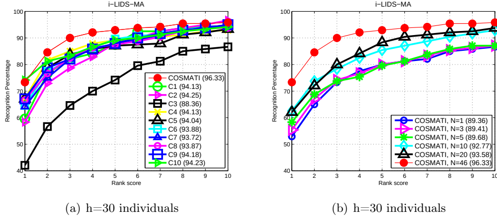
Figure 7.19: Performance comparison: (a) with models based on a single type of covariance descriptor; (b) w.r.t. the number of given frames
