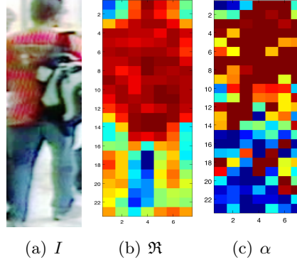
Figure 5.16: Illustration of patch significance: (a) one of many frames obtained during tracking; (b) reliability map obtained by the first method; (c) confidence map obtained by boosting. Colours correspond to significance of patches (for clarity only \frac{W}{4} \times \frac{W}{4} patches, shifted by \frac{W}{8} pixels are illustrated, red indicates the highest significance, blue the lowest).
