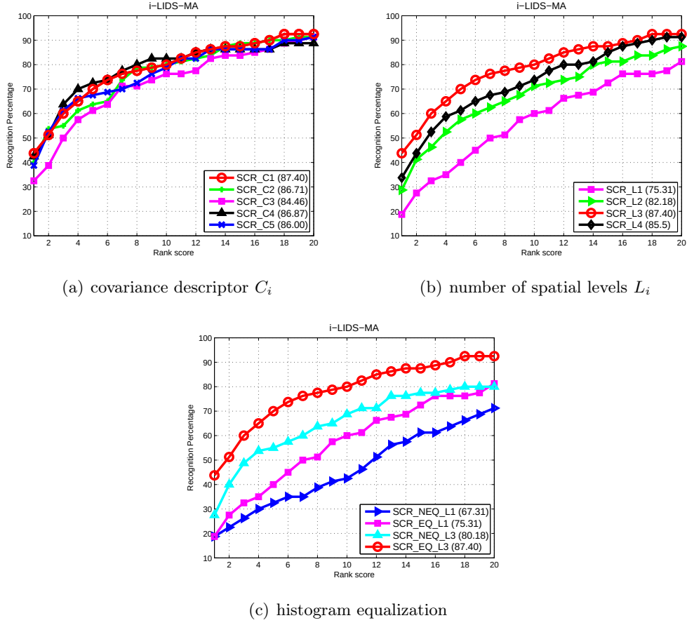
Figure 7.12: CMC curves obtained on i-LIDS-MA dataset using SCR signature: (a) performance comparison of different covariance descriptors; (b) analysis of the level's depth: L1 corresponds to the matching using only one level (level 0 refers to the full body, see figure 4.11), L2 corresponds to the matching using two levels (level 0 and level 1), etc. ; (c) the performance of SCR signature with and without histogram equalization (HE vs. NHE).
