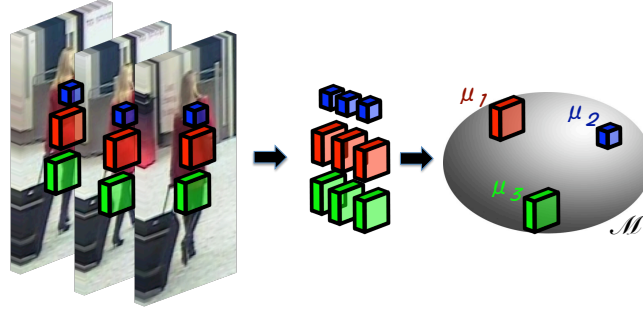
Figure 5.14: Computation of three MRC patches. Covariances gathered from tracking results are used to compute the mean covariance using Riemannian manifold space (depicted with the surface of the sphere). The mean covariance forms MRC patch.
