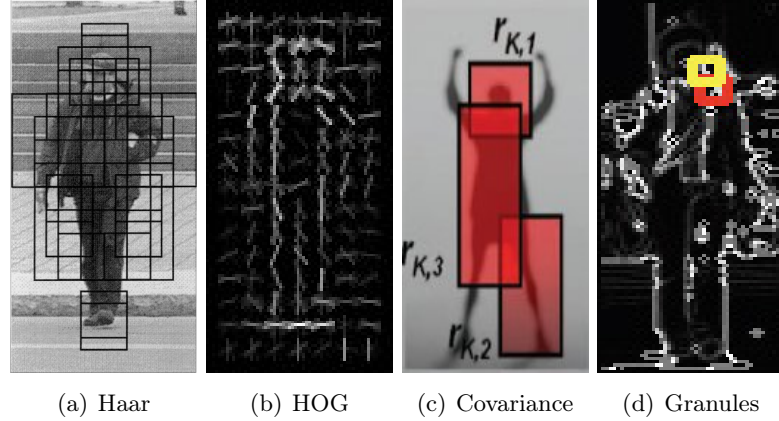
Figure 3.4: Human detection approaches: (a) Haar wavelets [Papageorgiou 2000]; (b) HOG descriptor weighted by the positive SVM weights [Dalal 2005]; (c) three possible covariance descriptor sub-windows [Tuzel 2008]; (d) granules comparing gradient orientations [Duan 2009].
