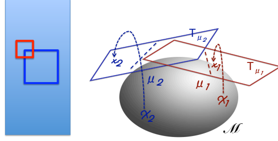
Figure 5.15: MRC Classifier. The manifold is depicted with the surface of the sphere, and the planes are the tangent spaces of the mean covariances. The samples \mathbf{x}_i are projected to tangent space T_{\mu_i} at means via \log_{\mu} operation.
