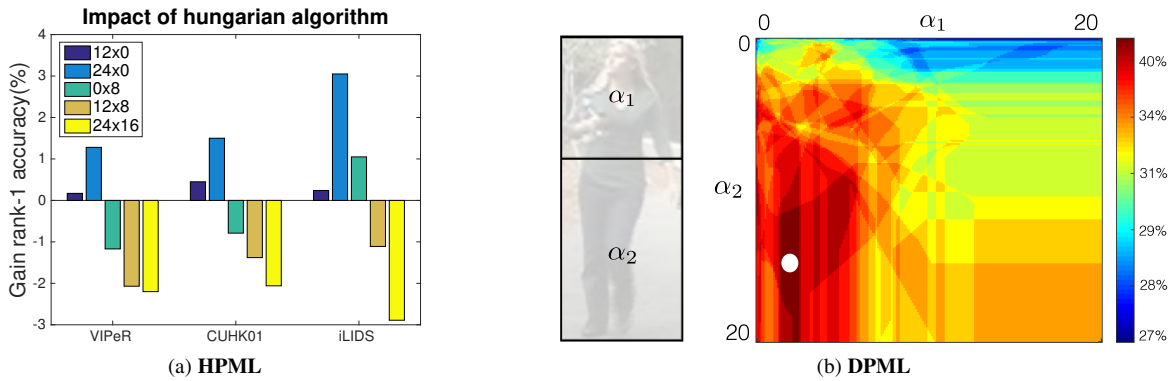
Fig. 15: Deformable model parameters: (a) HPML – comparison of different allowable neighborhoods (horizontal×vertical) when applying Hungarian algorithm for matching patches; (b) DPML – exhaustive grid search over \alpha_1 and \alpha_2 coefficients for VIPeR. \alpha_1 and \alpha_2 correspond to patches locations w.r.t. to the left image. Grid search map illustrates Rank-1 recognition rate as a function of (\alpha_1, \alpha_2) . The white dot highlights the optimal operating point.
