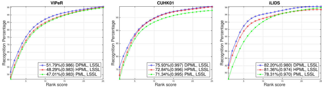
Fig. 16: Performance comparison of Patch based Metric Learning ( PML ) with our deformable models: unsupervised HPML and supervised DPML . Rank-1 identification rates as well as nAUC values provided in brackets are shown in the legend next to the method name.
