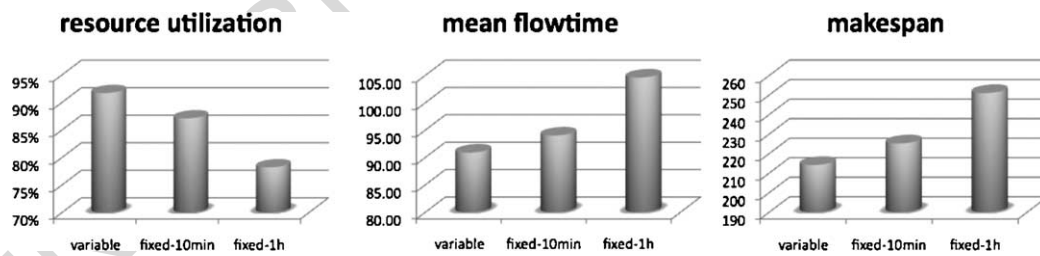
Fig. 10. Resource utilization, makespan and mean flow time for variable- and fixed-length slots approaches.
